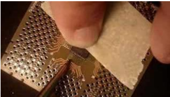
Hand Soldering .5mm QFN
