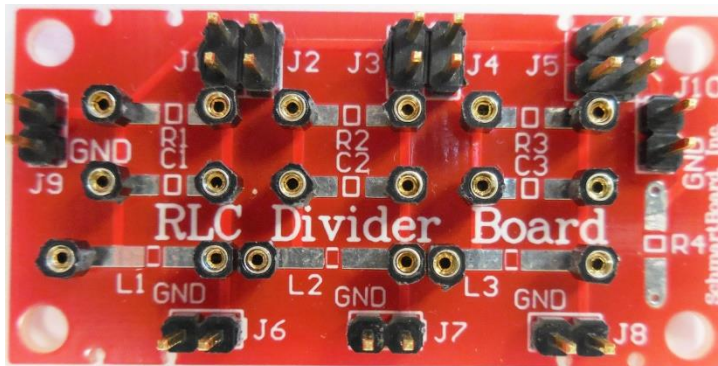
Schmartboard RLC Divider Board
