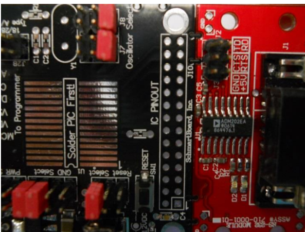
Top View of connected boards. These hold the boards, but glue is optional for a solid connection
