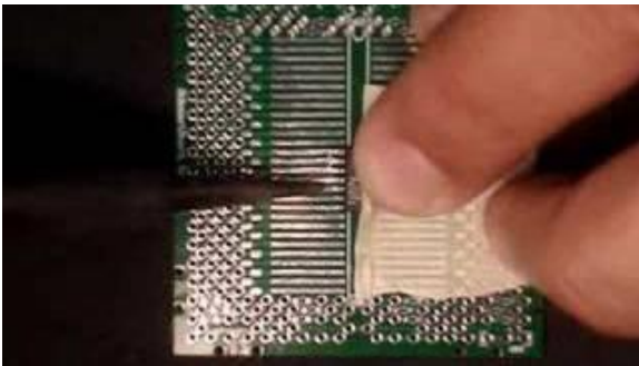
Hand Soldering an SOIC Part
