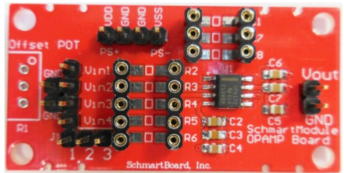
Schmartboard OpAmp Board
