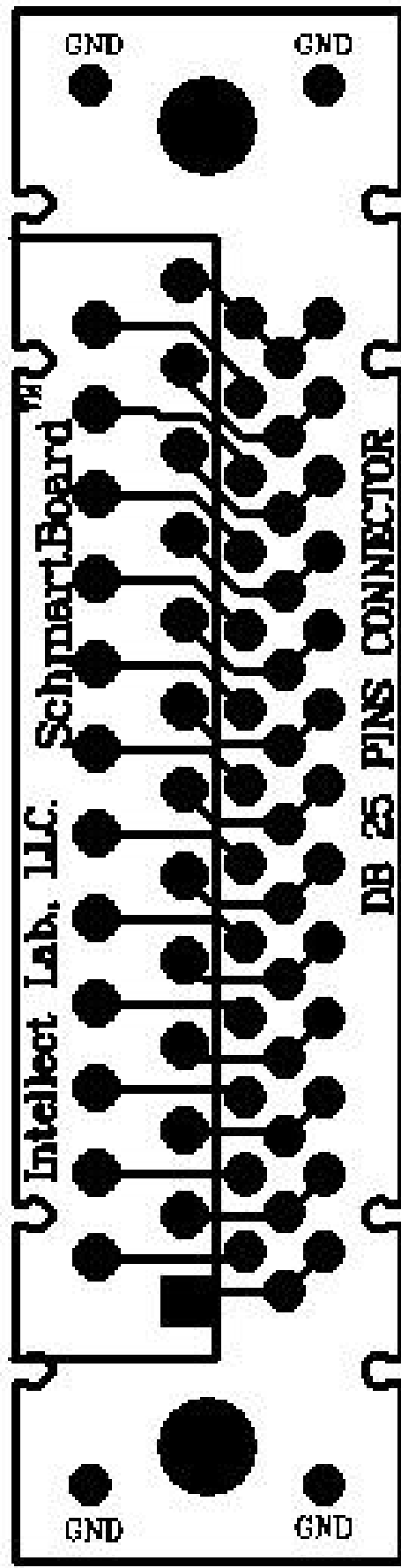
DB25 CONNECTOR (201-0104-01)
